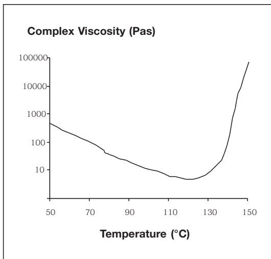
Rheology
